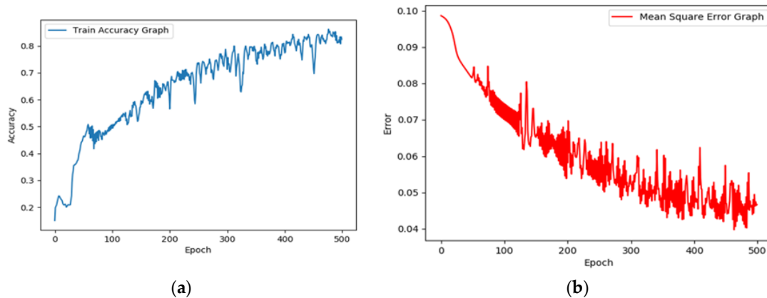
Figure 8. Accuracy and MSE of the CNN algorithm; (a) accuracy of the CNN rises continuously with every epoch; (b) MSE of CNN reduces with each epoch.
