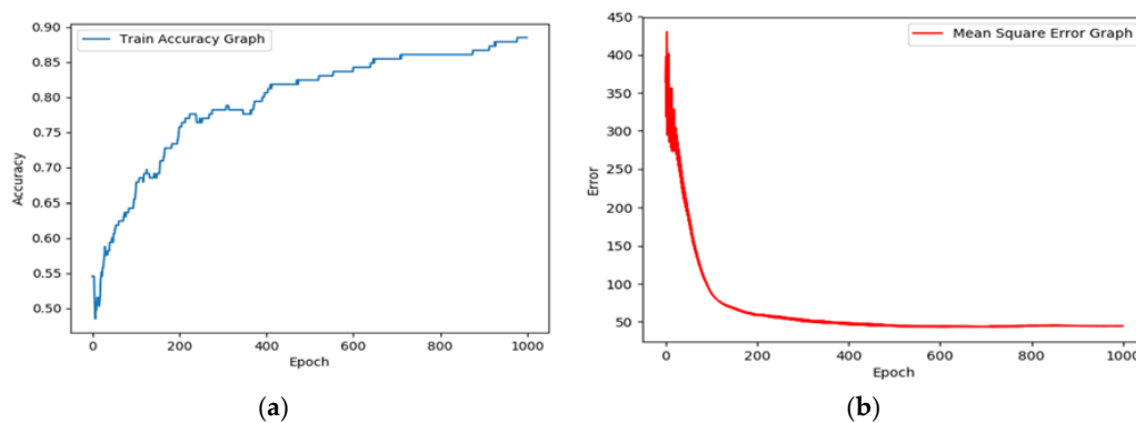
Figure 6. Accuracy and mean square error (MSE) graph of the MLP algorithm; (a) the accuracy of MLP increases as the number of epochs increases; (b) MSE reduces with every epoch and reaches the minimum point after 1000 epochs.
