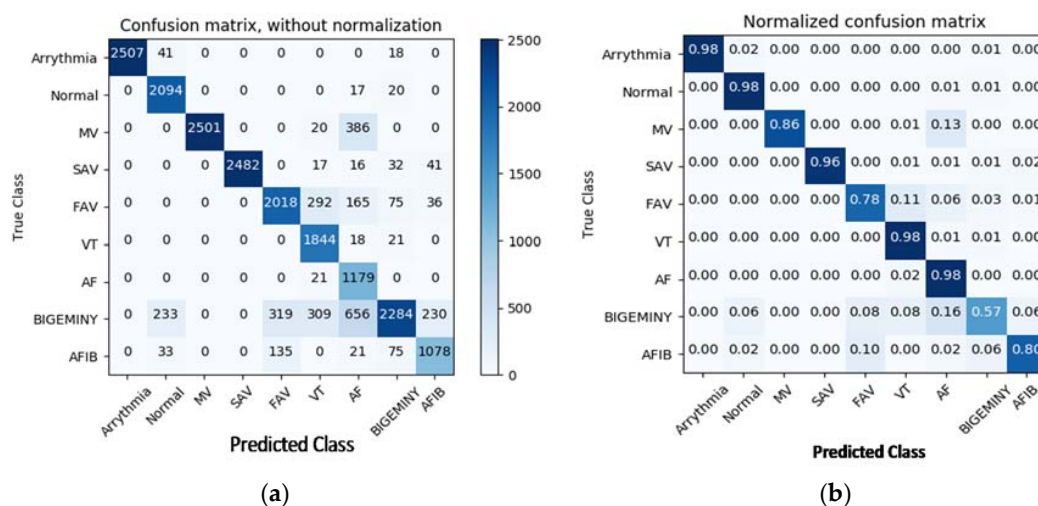
Figure 9. CM with and without normalization of the CNN algorithm; (a) most of the arrhythmia was correctly classified by CNN except bigeminy and FAV; those diseases might have the same characteristics as others; (b) normalized CM gives the accuracy of the CNN in percentage form.
