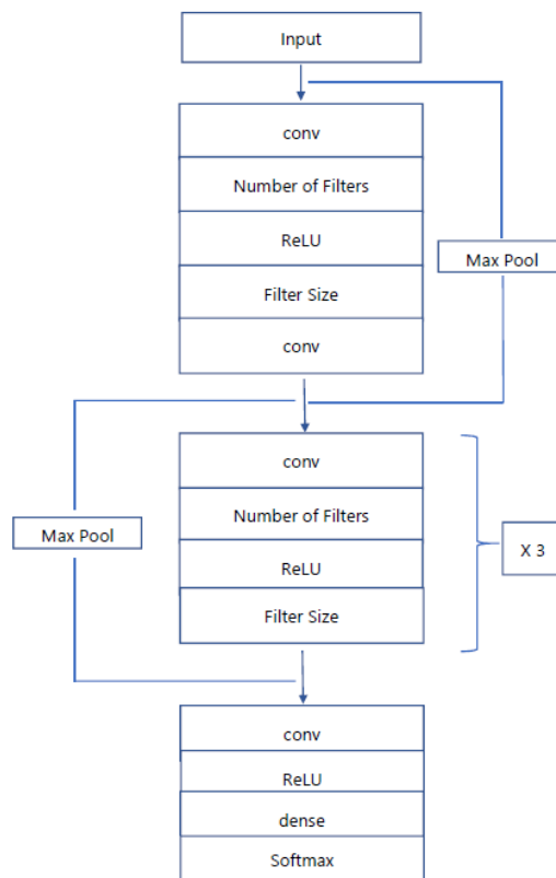
Figure 4. Proposed Algorithm of Convolution NN. Four convolutional layers were used. In addition, there is one output layer with a softmax layer to hold the output of the NN.
