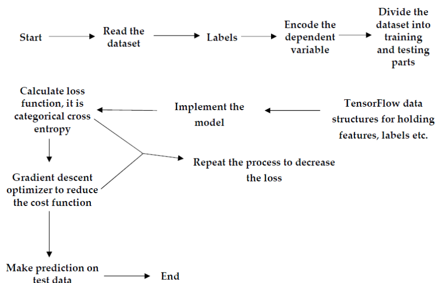
Figure 3. System process flowchart of Multilayer Perceptron (MLP) and Convolution NN. To define features and labels in the dataset, two TensorFlow variables were defined. One hot encoder was used to encode the dataset.
