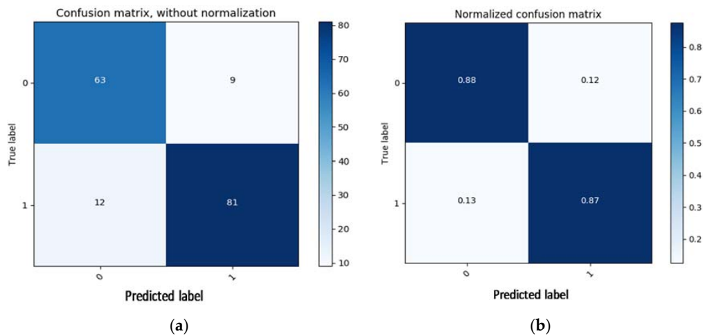
Figure 7. Confusion matrix (CM) with and without normalization of the MLP algorithm; (a) 63 arrhythmias and 81 normal signals are correctly classified, while 9 arrhythmias and 12 normal ECG signals are misclassified; (b) CM with normalization gives an accuracy in percentage; in this case, accuracy was 88% for arrhythmia and 87% for normal sinus ECG.
